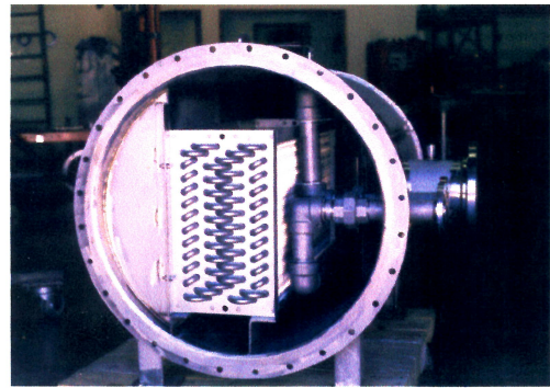
Custom Designed CDC "COOLER" Package's built to order
